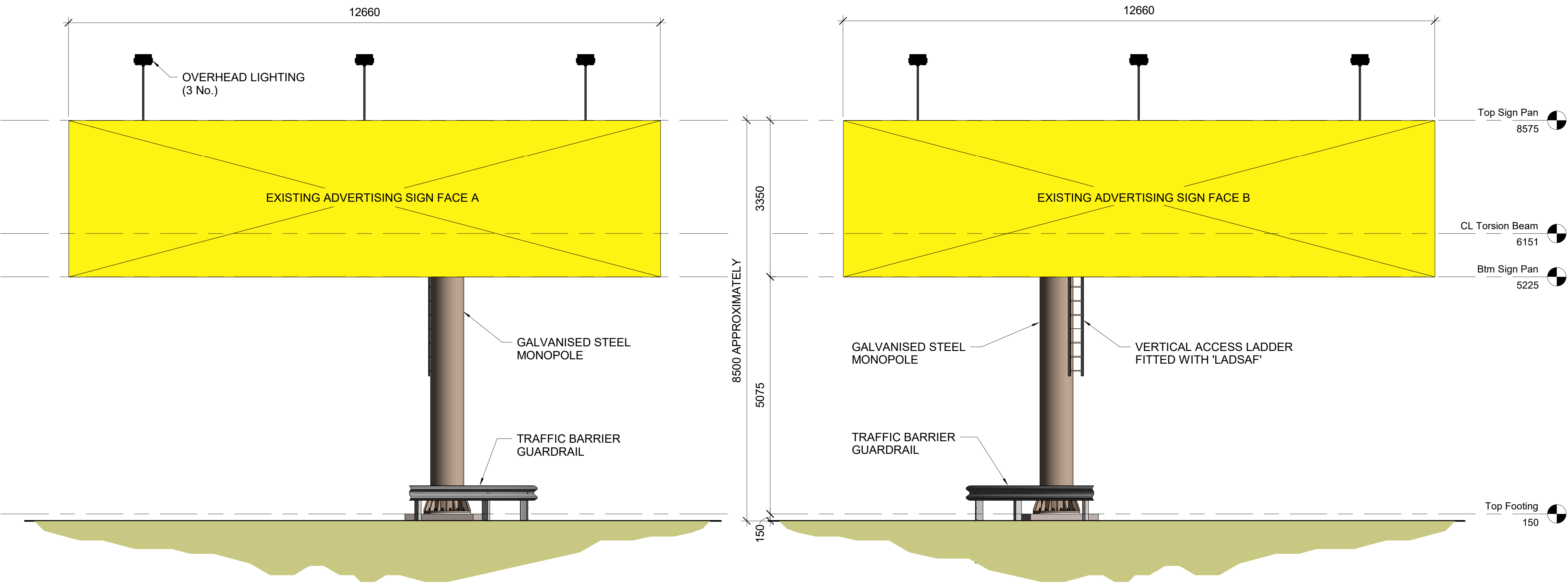
EXISTING ADVERTISING SIGN FACE A ELEVATION SCALE 1 : 50
