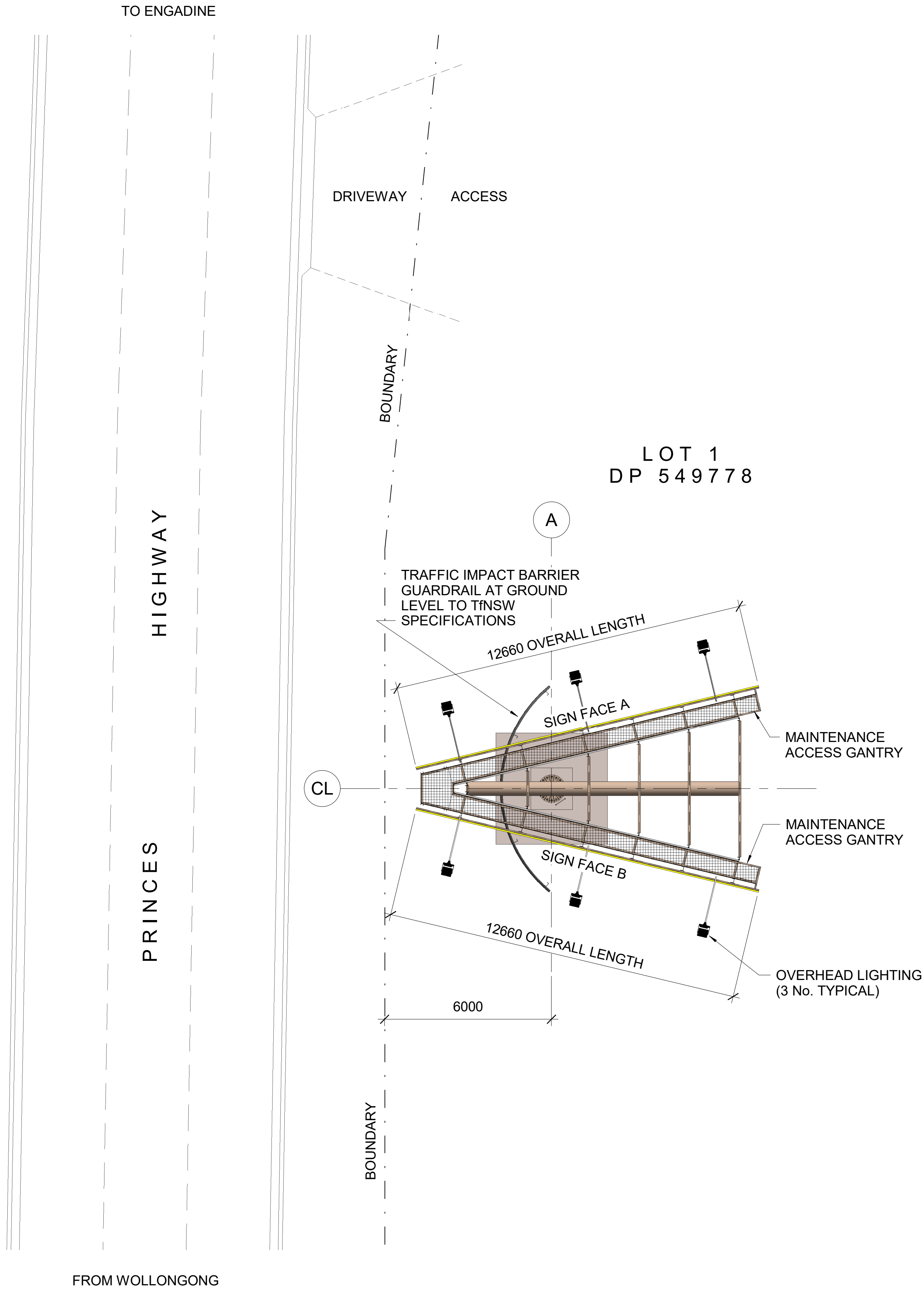
EXISTING ADVERTISING SIGNAGE PLAN SCALE 1 : 100
